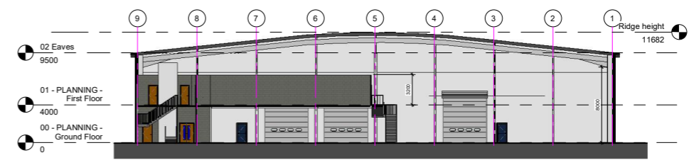
8 PLANNING - Section 1 1 : 200
