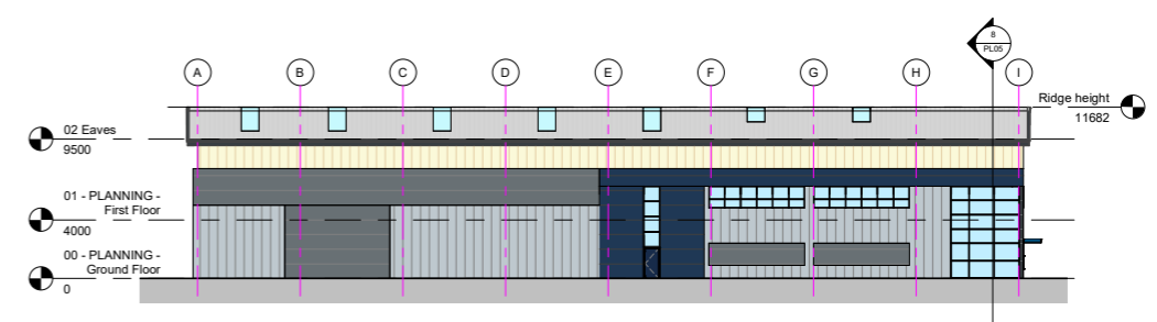
6 PLANNING - Side Elevation (1) 1 : 200
