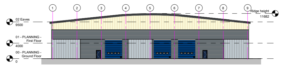
5 PLANNING - Rear Elevation 1 : 200
