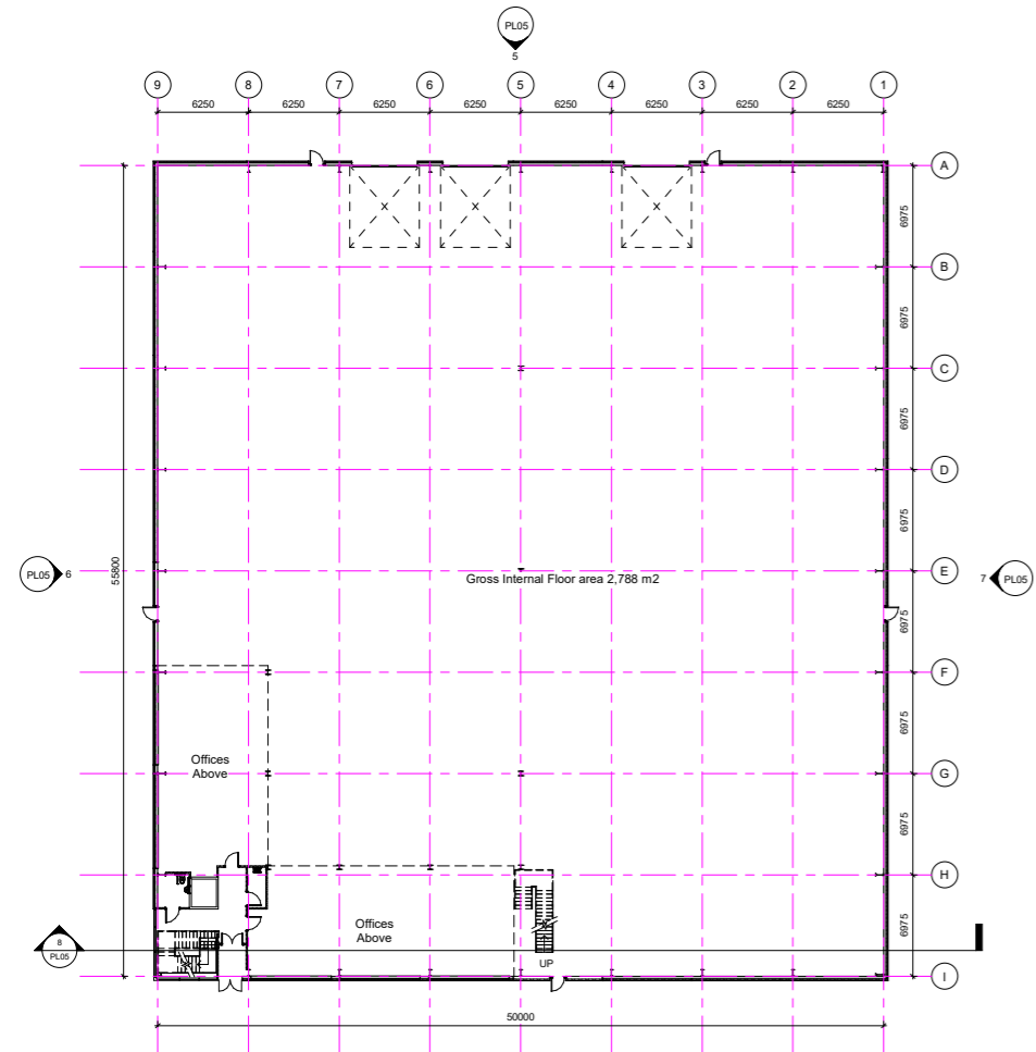
00 - PLANNING - Ground Floor 1 : 200
