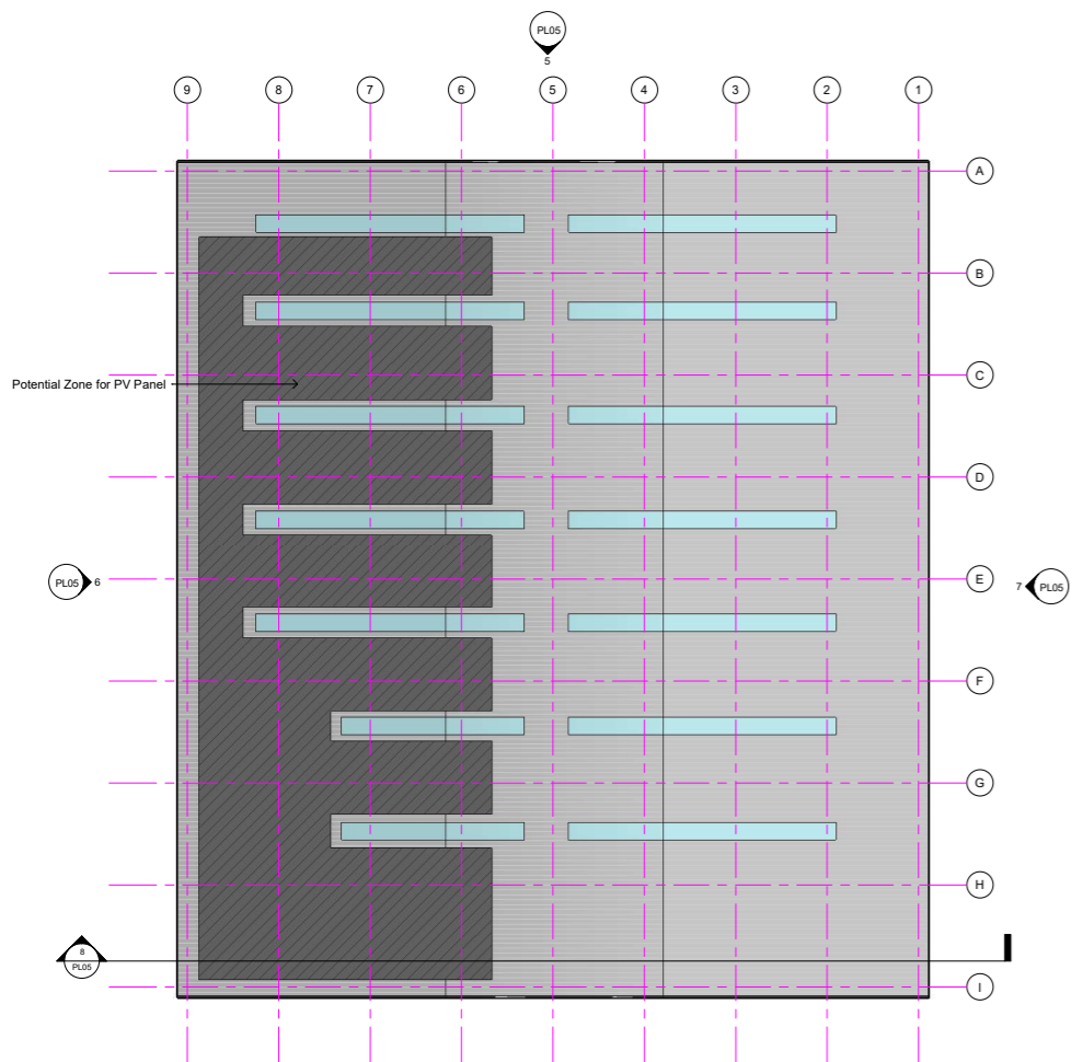
02 - PLANNING - Roof Plan 1 : 200
