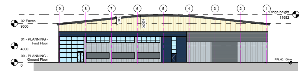
4 PLANNING - Front Elevation 1 : 200
