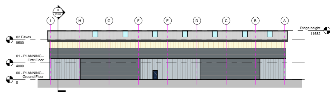
7 PLANNING - Side Elevation (2) 1 : 200
