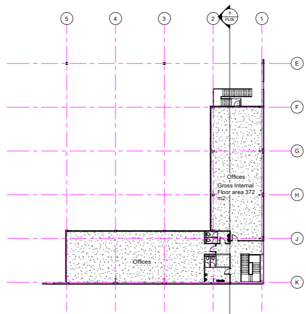
2 01 - PLANNING - First Floor 1 : 200
