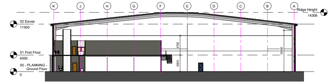
8 PLANNING - Section 1 1 : 200
