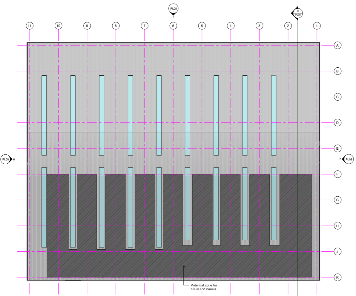
3 02 - PLANNING - Roof Plan 1 : 200
