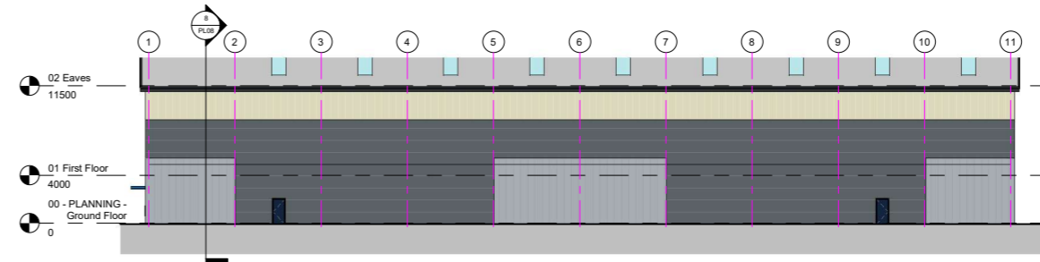
5 PLANNING - Rear Elevation 1 : 200
