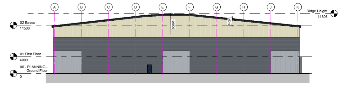
6 PLANNING - Side Elevation (1) 1 : 200
